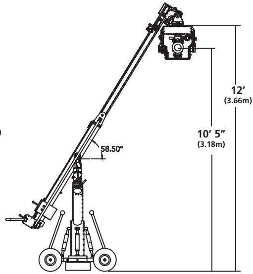
Underslung Extended
