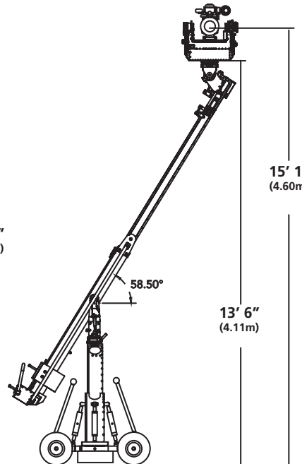
Overslung Extended
