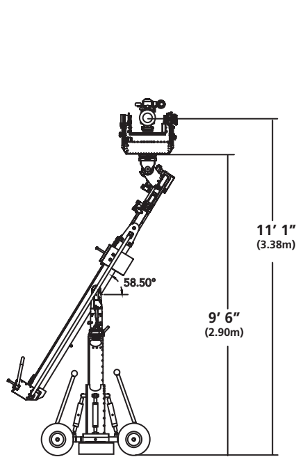
Overslung Retracted
