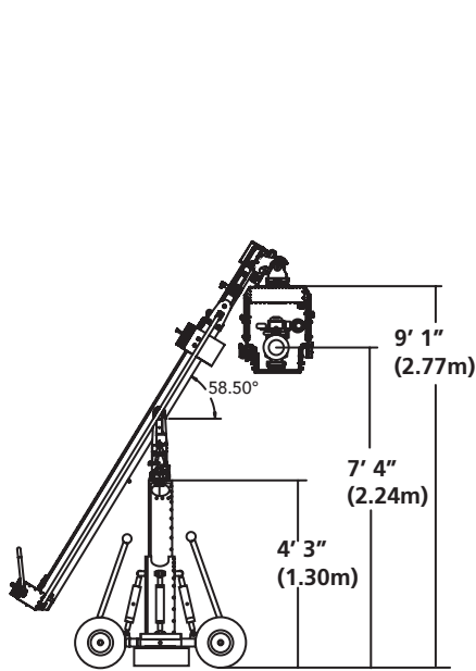
Underslung Retracted
