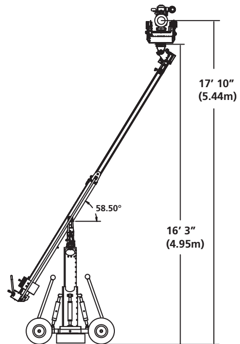
Overslung Extended
