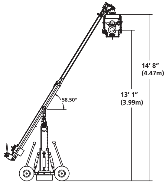
Underslung Extended
