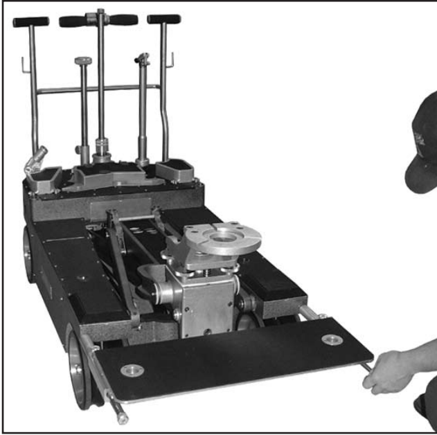
The Front Board attaches with two thumb screws.
