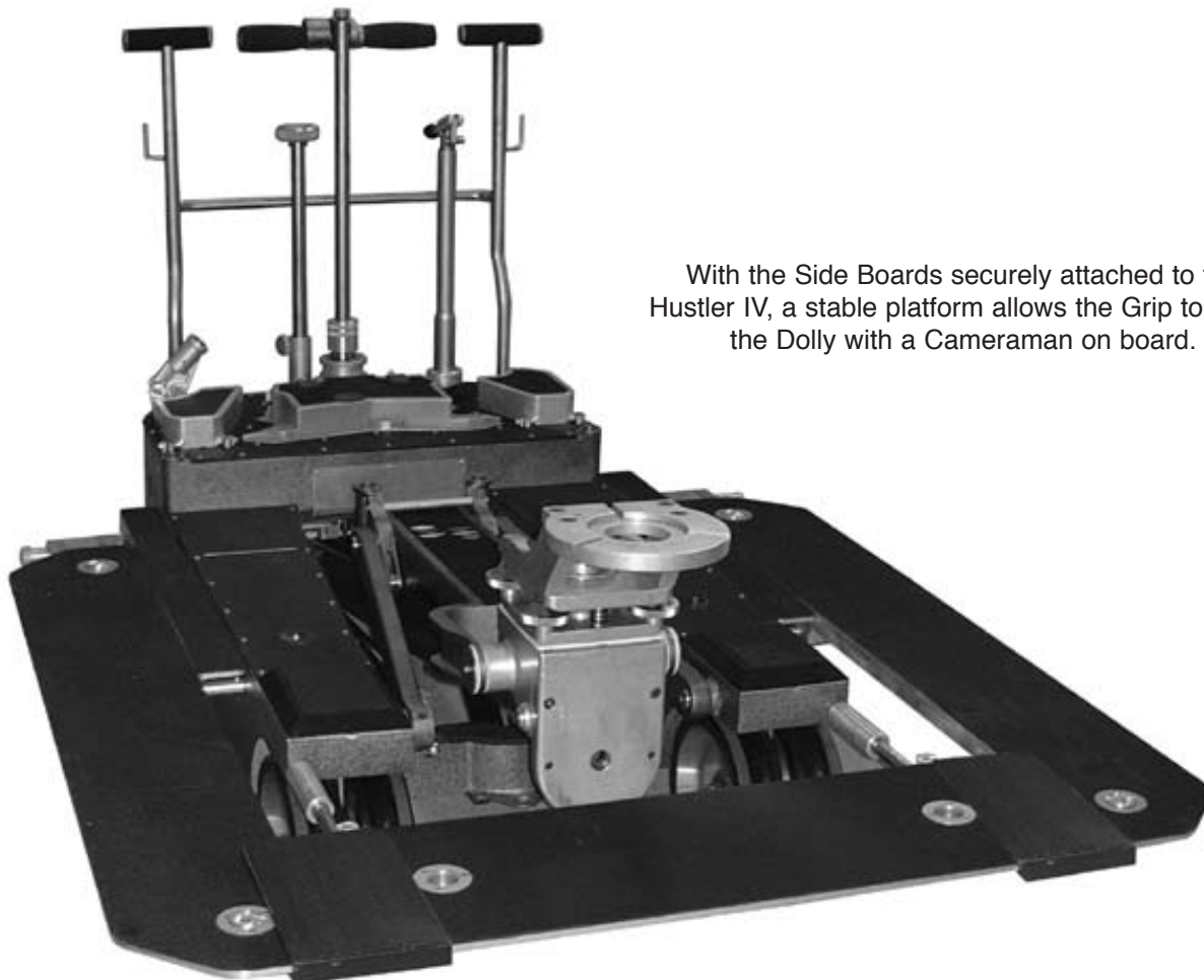
The Side Boards attach to either side of the Hustler IV. They slide into place and are secured to the chassis with two thumb screws.
