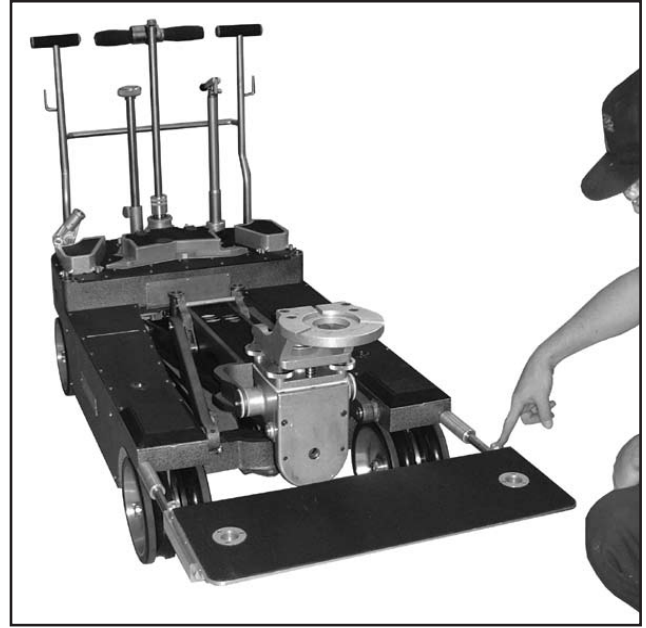
The Front Board may be retracted or extended.
