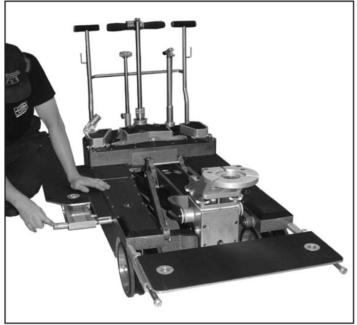
The Side Boards may be moved to the rear of the Dolly for easy access to the front thumb screw. Then move the board forward to access the rear thumb screw.
