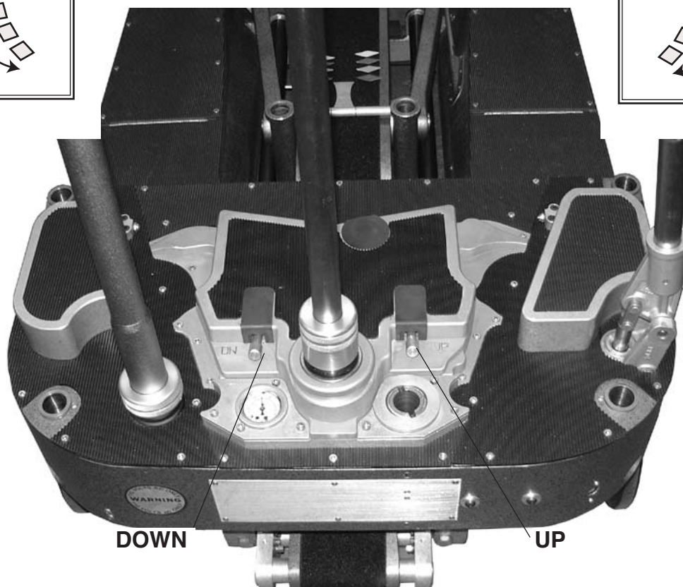
Looking down while standing at the rear of the Dolly. Control Valve Handle and Steering Handle removed for clarity.
